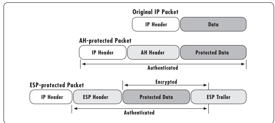
Figure 1: AH and ESP components of IPsec
