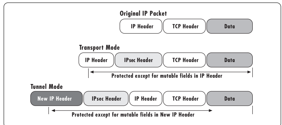
Figure 2: IPsec transport and tunnel modes
